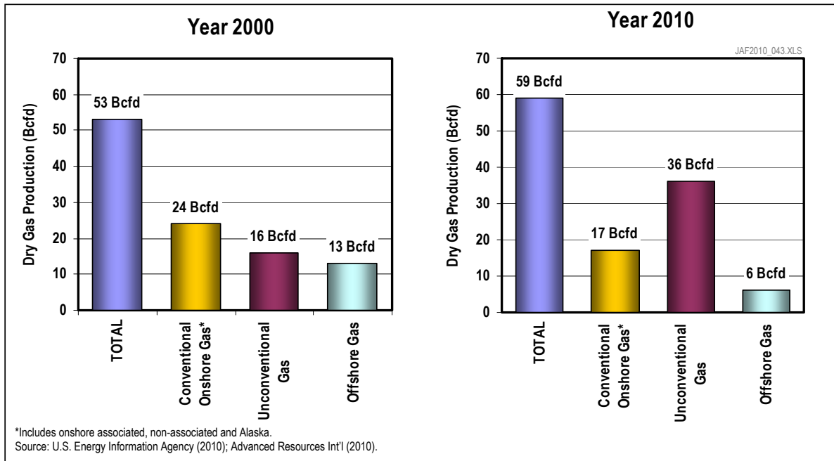
Figure I-1. Unconventional Gas Has Become the Dominant Source of U.S. Natural Gas Supply
