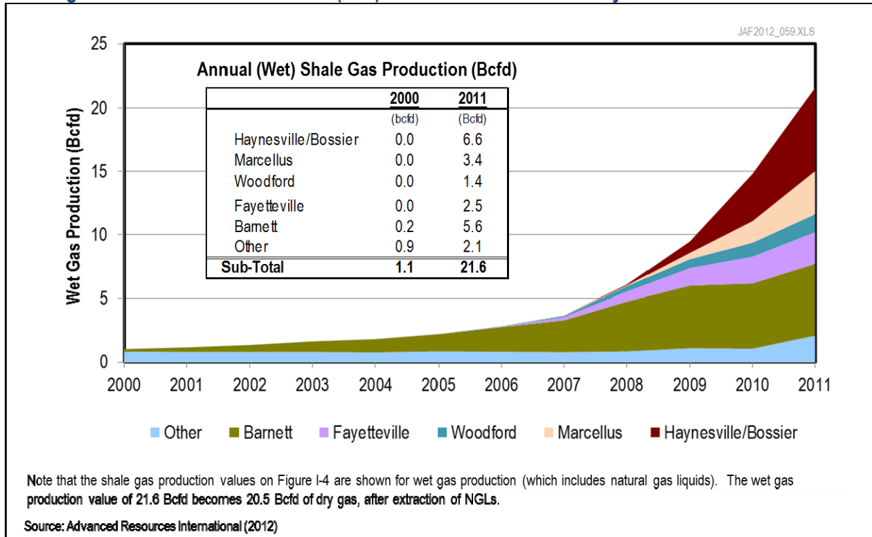
Figure I-4. Shale Gas Production (Wet) Has Increased Dramatically in the Past Ten Years
