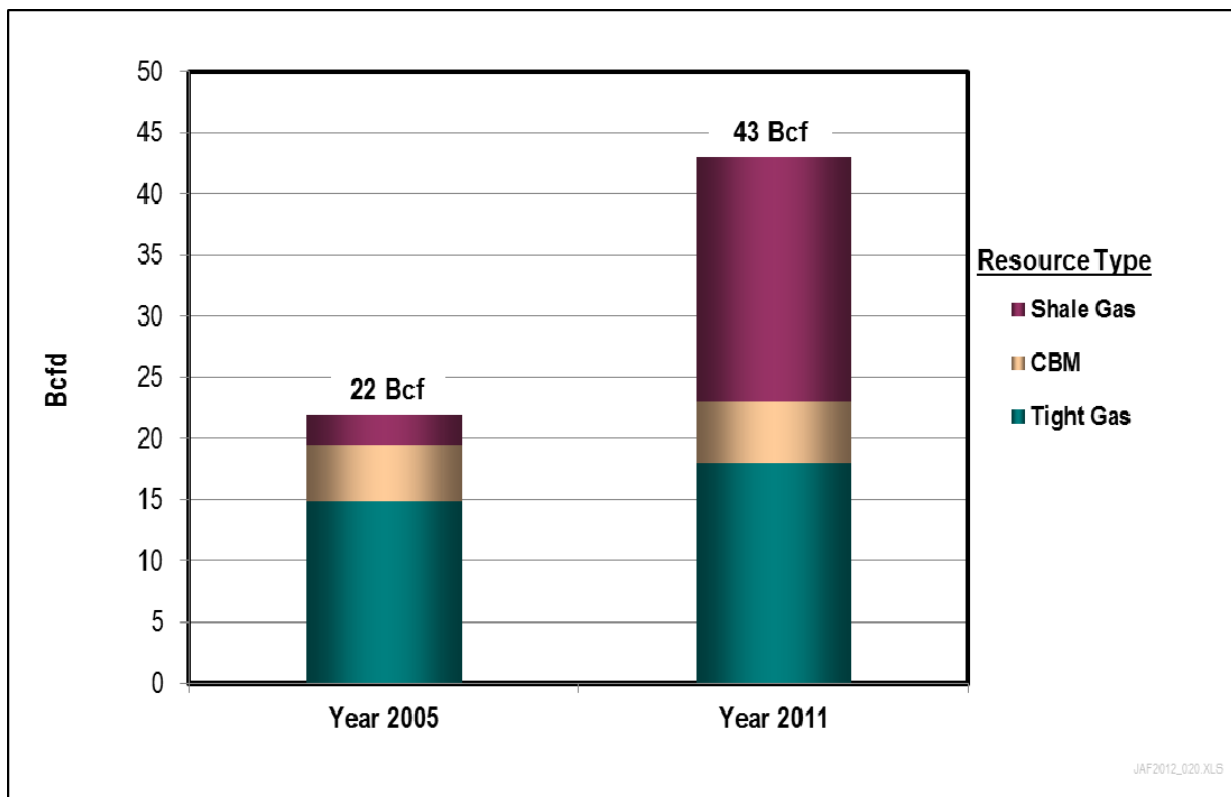
Figure I-3. Changes in Unconventional Dry Natural Gas Production by Resource Type
