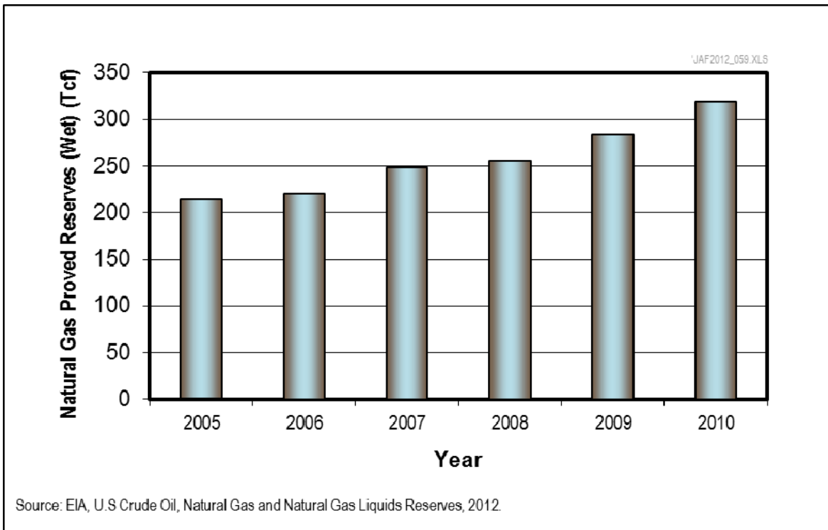
Figure I-2. Natural Gas Proved Reserves (Wet) Have Risen Sharply in the Past Five Years
