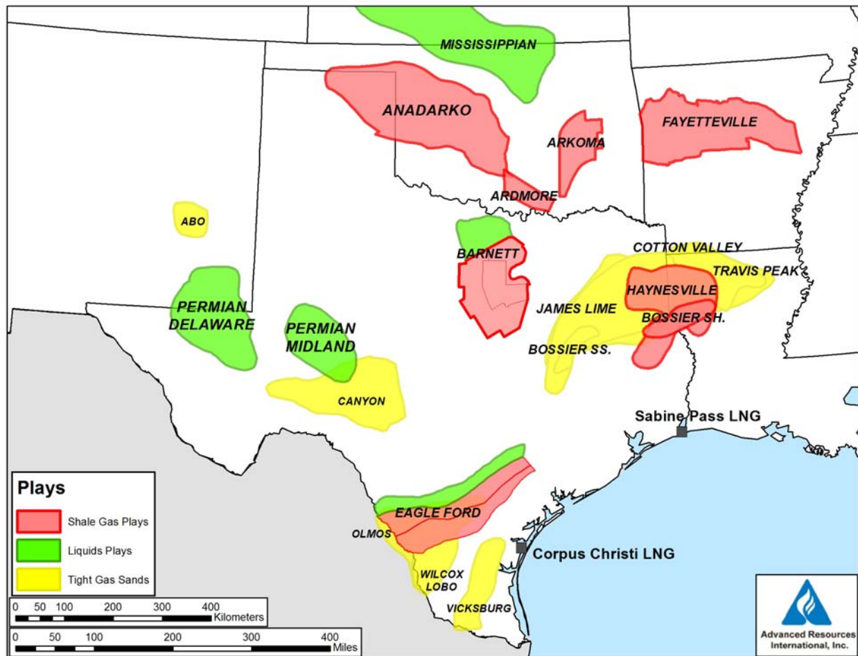
Figure VI-1. Location of Unconventional Gas Plays: “Corpus Christi Supply Area”
