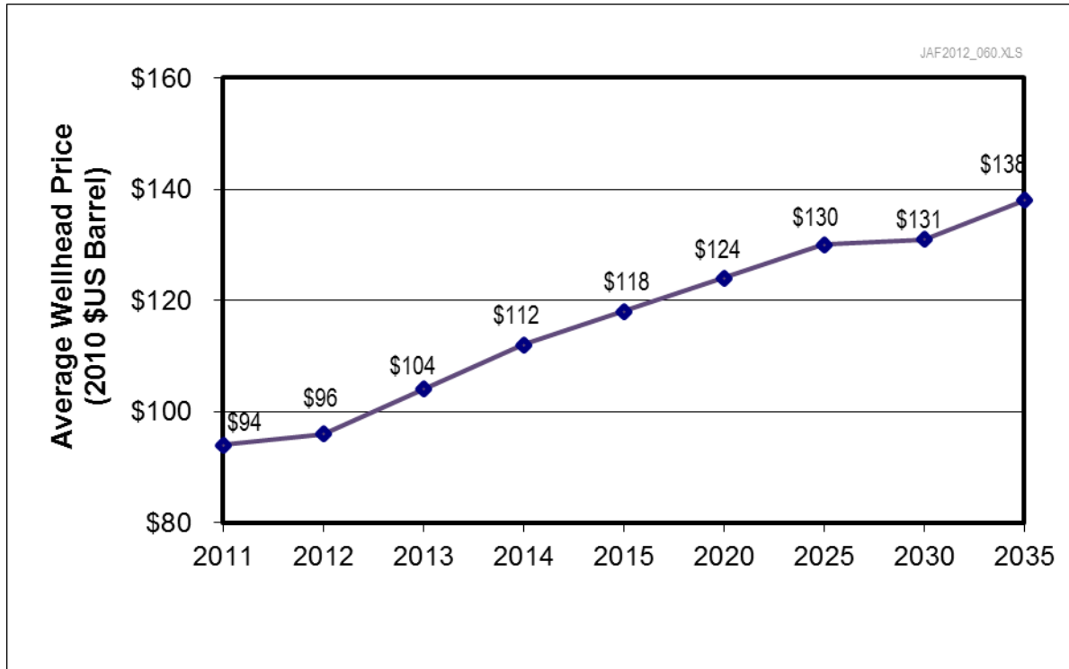
Figure III-3. Reference Case Oil Prices, AEO 2012
