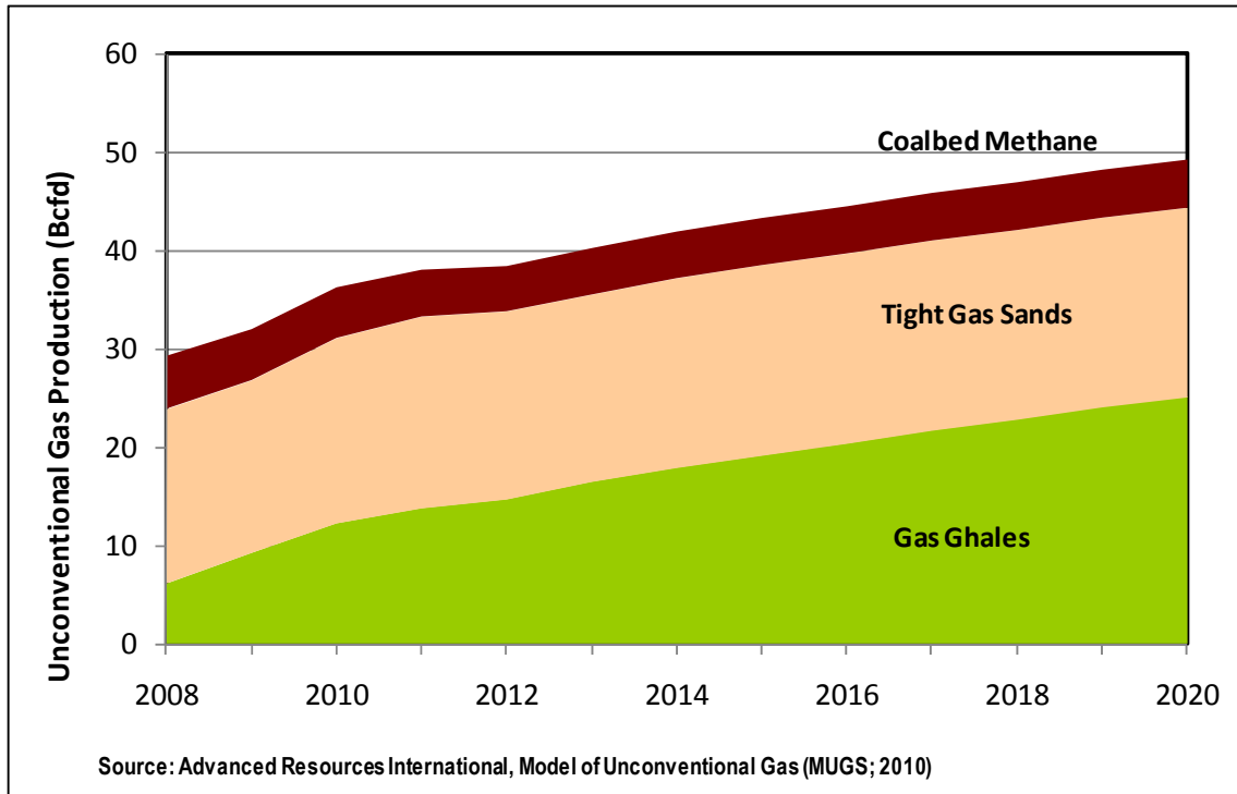
Figure IV-1. Mid-Term Expectations for Unconventional Gas Productive Capacity
