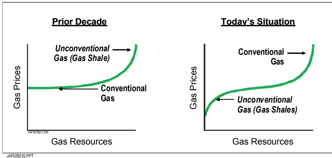
Figure II-3. Today's Domestic Natural Gas Price/Supply Curve
