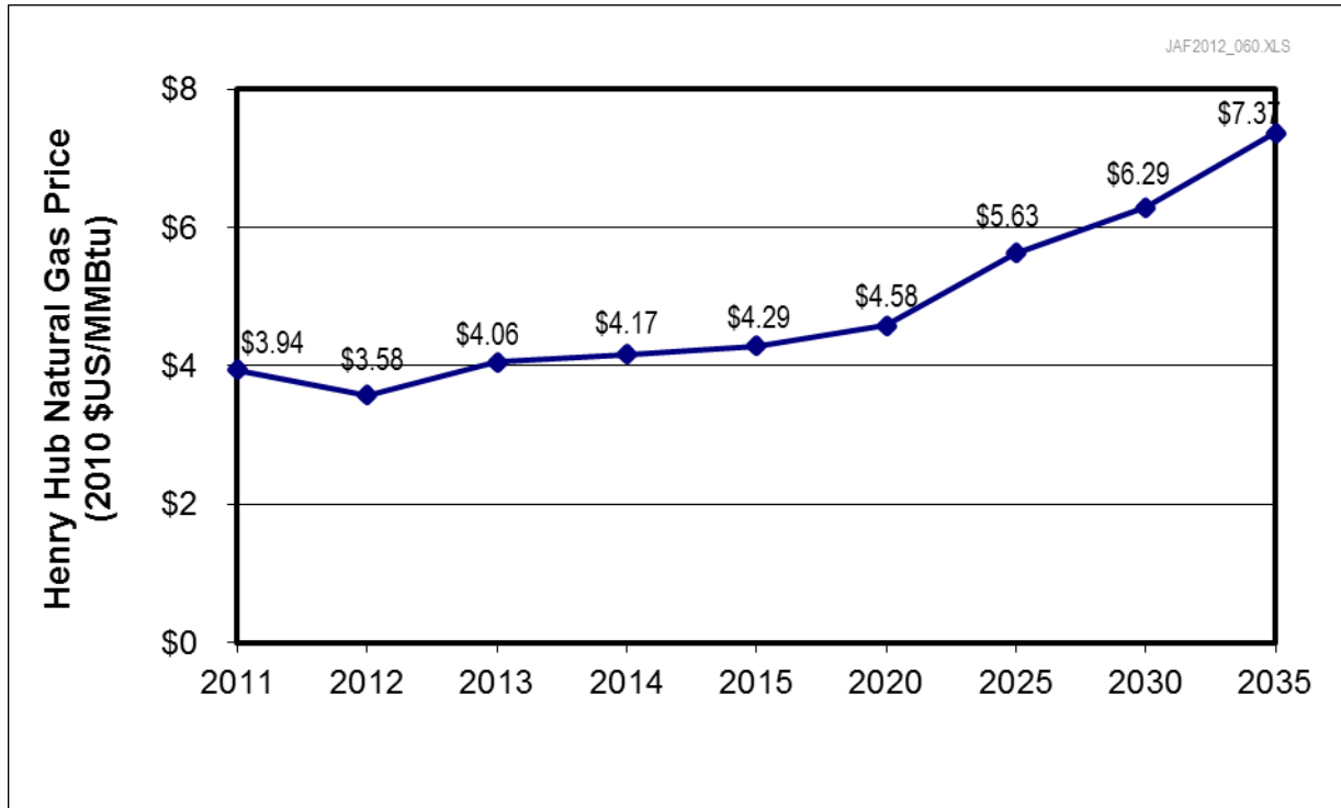
Figure III-2. Reference Case Natural Gas Prices, AEO 2012
