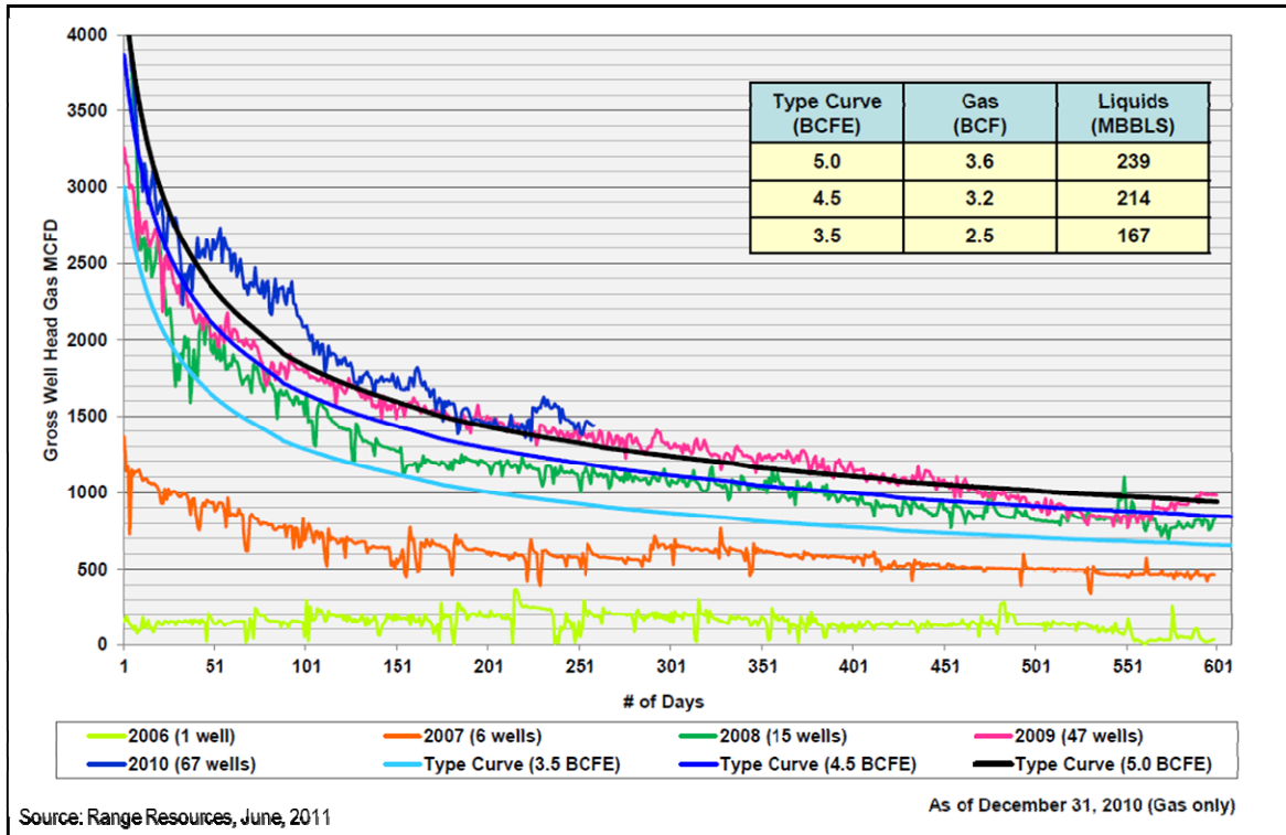
Figure V-4. Improvements in Shale Well Performance: Range Resources
