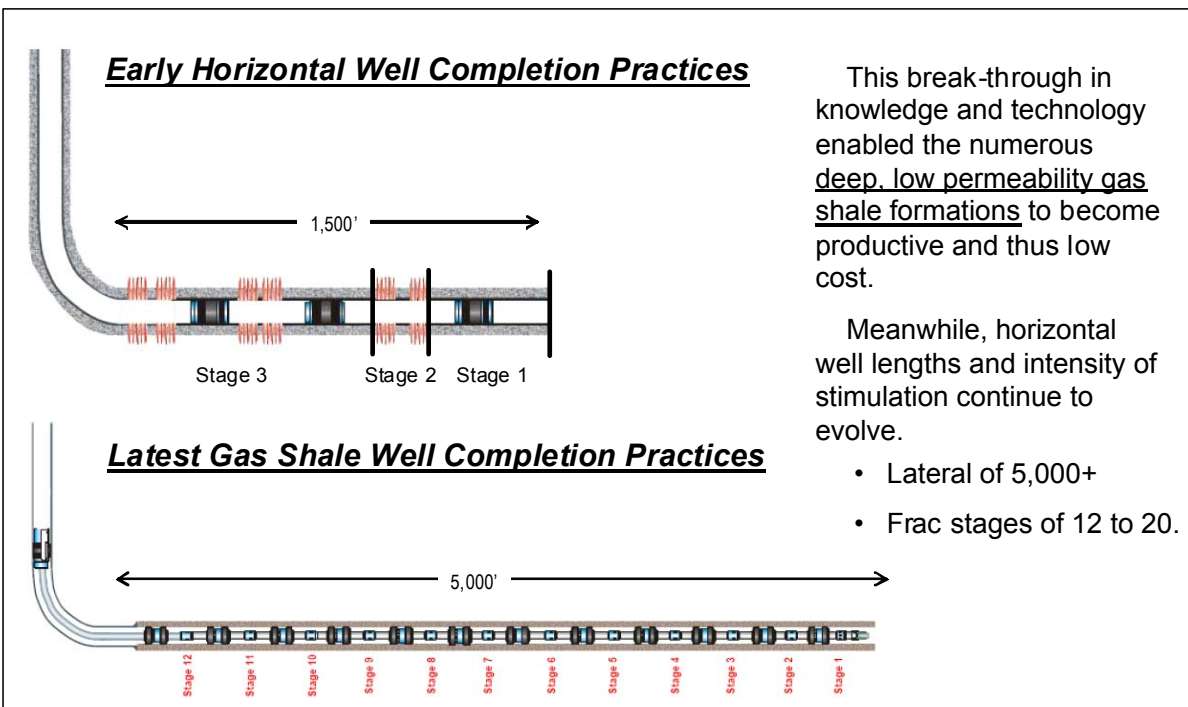
Figure V-2. Changes in Well Completion Practices
