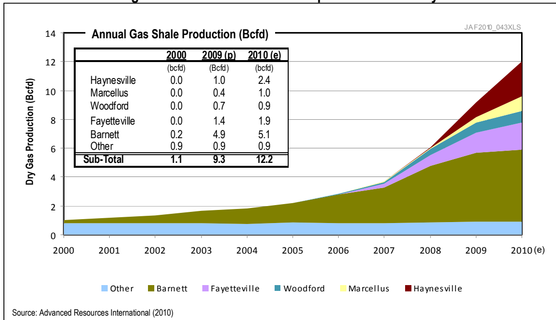
Figure I-4. Gas Shales Drive “Expectations of Plenty”
