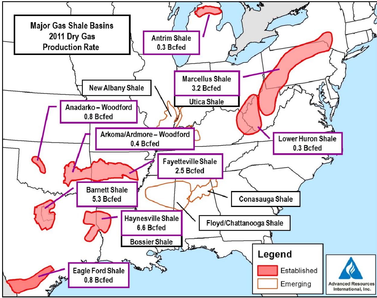
Figure II-2. Locations of Established Shale Gas Basins*
