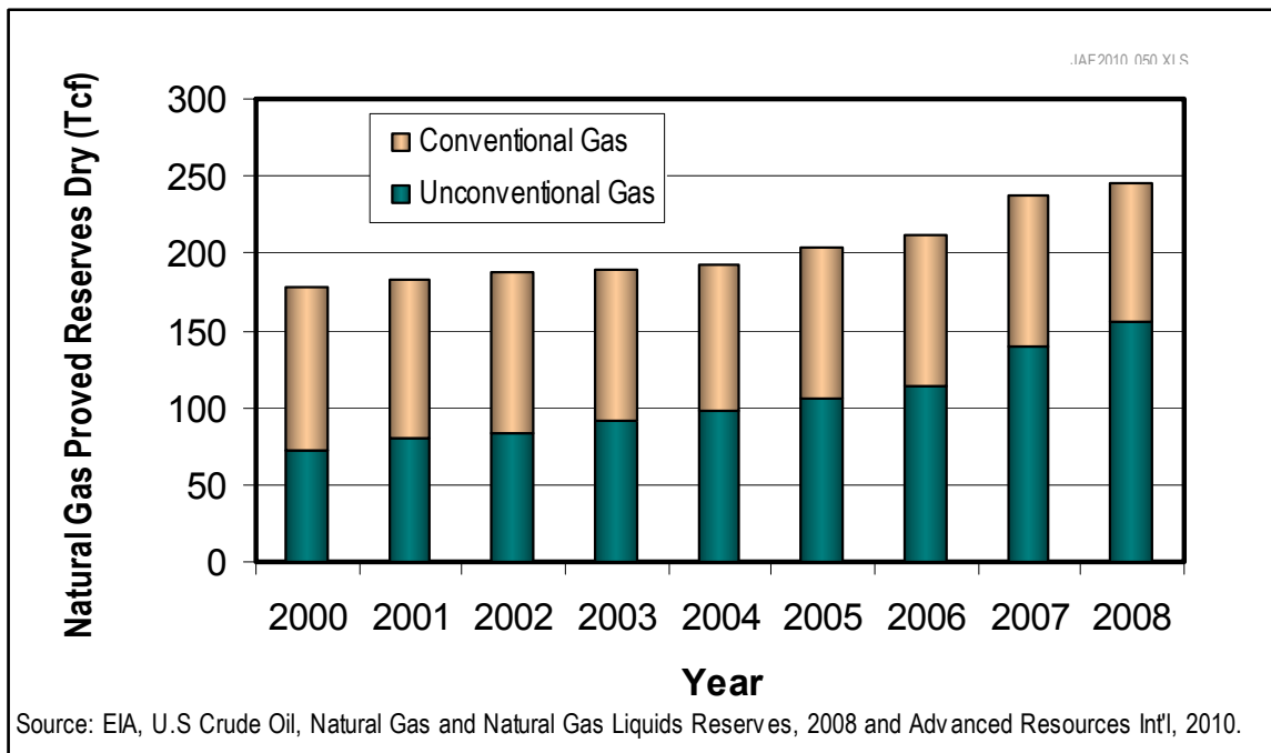
Figure I-2. A Decade of Increases in Domestic Natural Gas Proved Reserves
