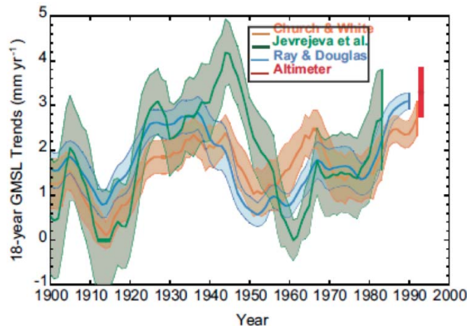
Figure 3.14 18-year trends of global mean sea level rise estimated at 1-year intervals. The time is the start date of the 18-year period, and the shading represents the 90% confidence. The estimate from satellite altimetry is also given, with the 90% confidence given as an error bar. [AR5 WGI Figure 3.14]
